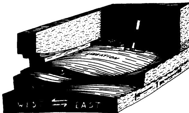
Fig. 11. Three-dimensional geometry of extensional composite structure, where shear bands (C) transect the mylonitic foliation (S). South of Golta.
