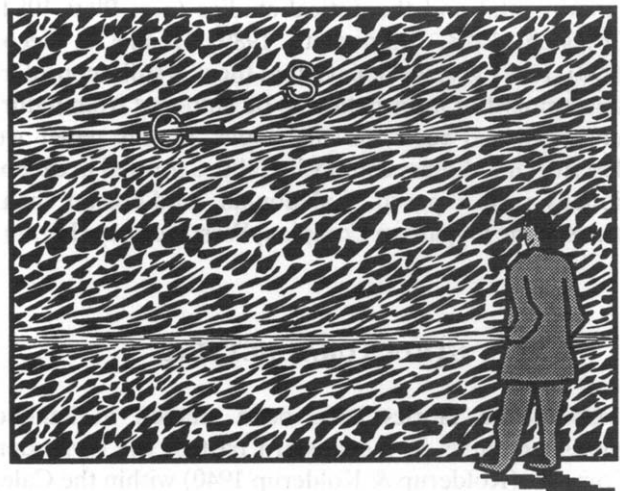
Fig. 2. Illustration of a mesoscopic composite structure similar to smaller-scale S-C structures. The foliation ( S ) is defined by flattened objects rotated into discrete shear zones ( C ). Idealized sketch based on observations of heterogeneously sheared agmatites, Golta.
