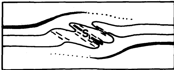
Fig. 9. Schematic diagram of a short fold train (contractional composite structure). The structure has a convex geometry with slip surfaces (black, weak layers) dipping in the direction of transport. Note the locally high angle between the internal foliation ( S_i ) and the weak layers. X-Z section, Toftøy.
