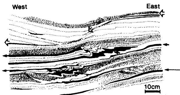
Fig. 10. Shear band (open arrows) linking two terminating micaceous layers in the upper part of the figure (extensional composite structure). The lower part displays contractional composite structures linking horizons marked with black arrows. Arrows indicate slip directions. X-Z section, Toftøy.
