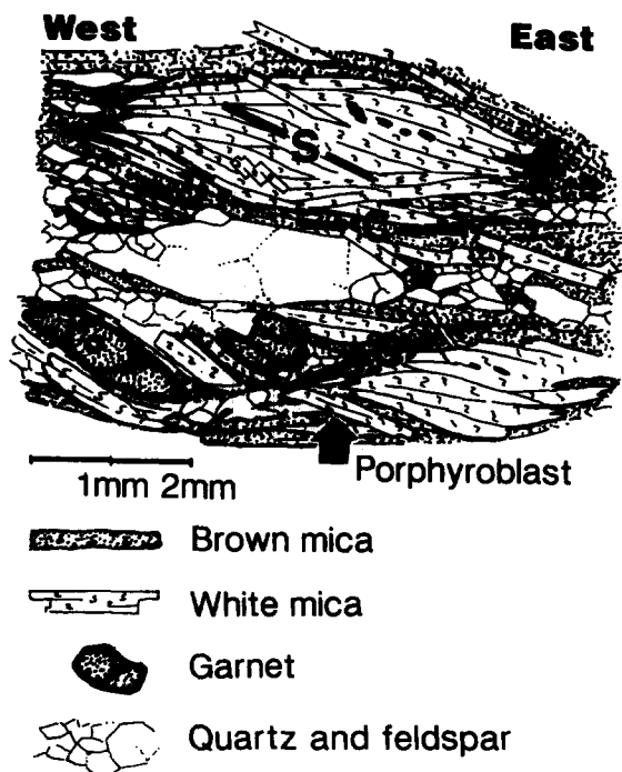
Fig. 4. Type II S-C structure. Note porphyroblasts of white mica (arrow) inclined to mica-fish. Both oblique growth of white mica during deformation and back rotation related to shear band formation is responsible for the S-C fabric. From high strain zone at Golta.
