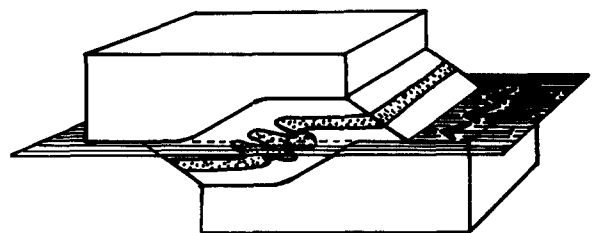
Fig. 14. Illustration of slip transfer across locally dipping layers, e.g. behind a tectonic lens. The evolving folds and possibly reverse-slip surfaces may in this case be termed reverse-slip crenulations , using Dennis & Secor's (1987) terminology.
